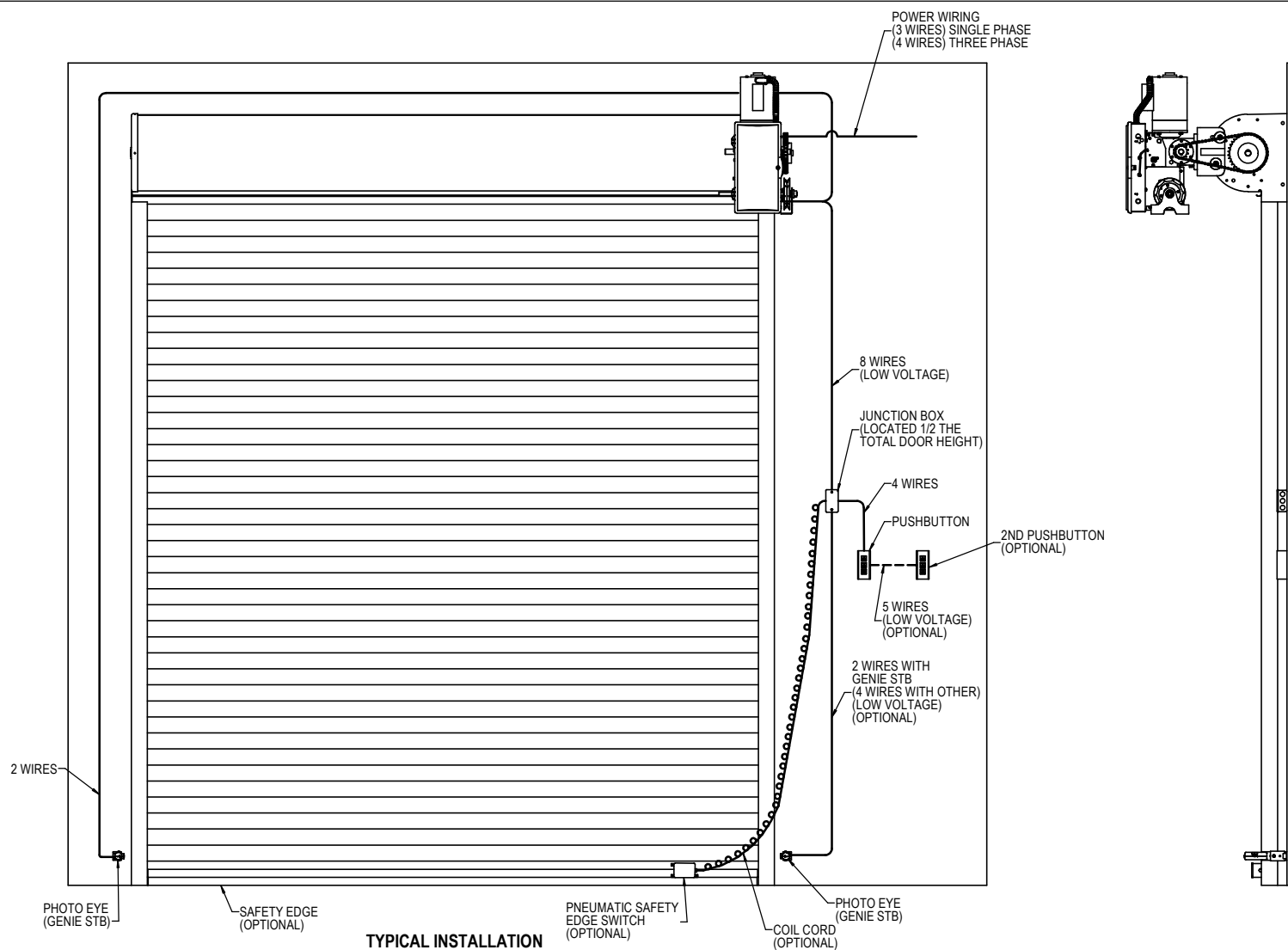
TYPICAL INSTALLATION
