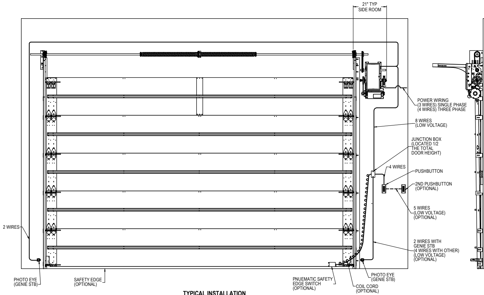
TYPICAL INSTALLATION
