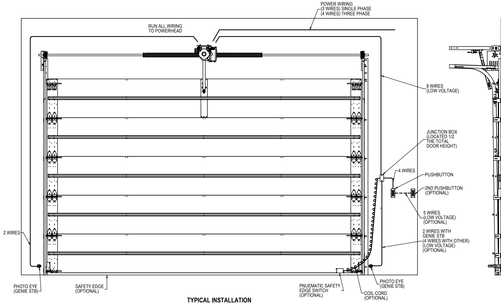
TYPICAL INSTALLATION
