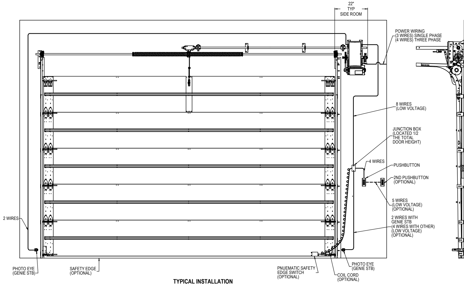
TYPICAL INSTALLATION
