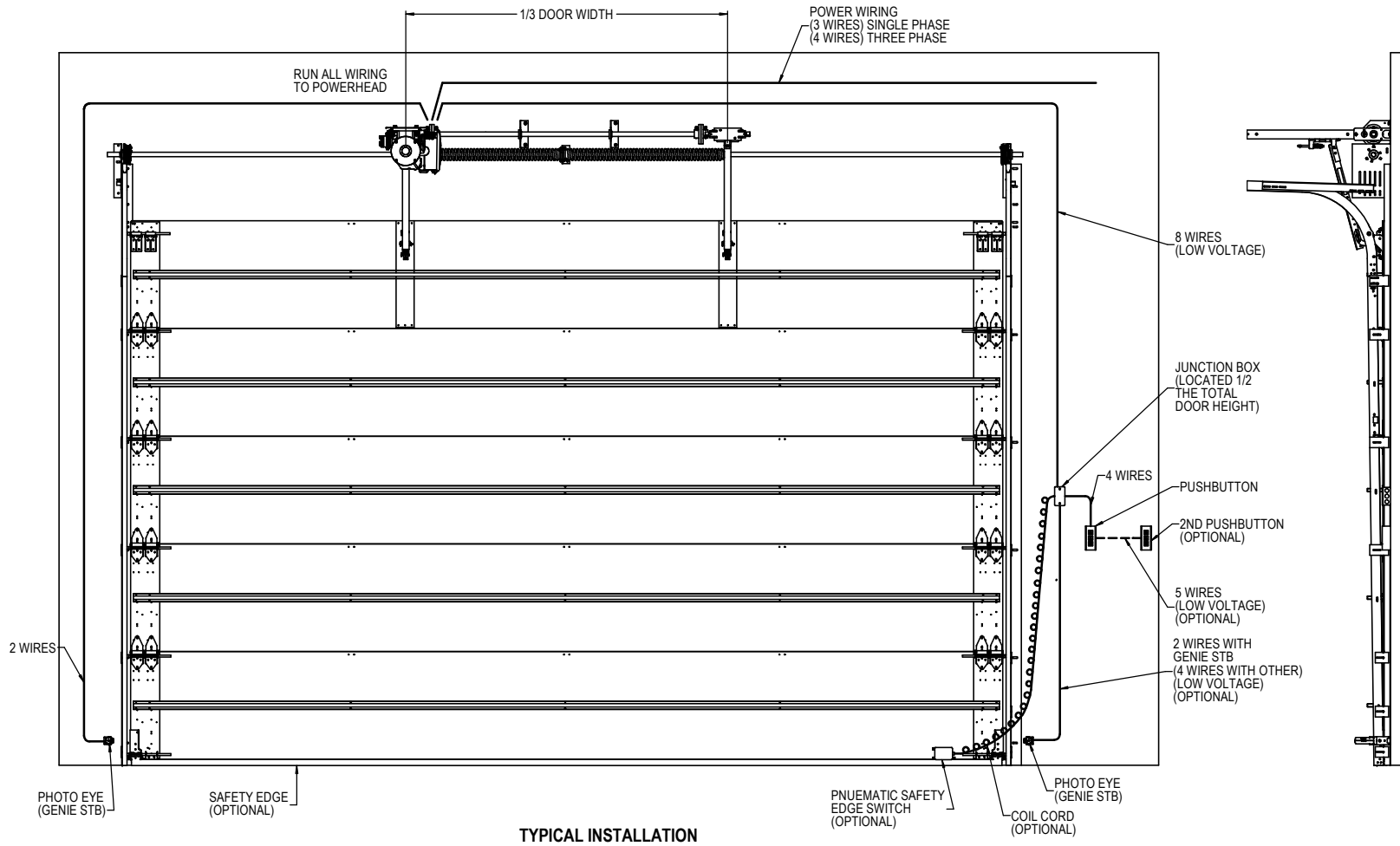
TYPICAL INSTALLATION
