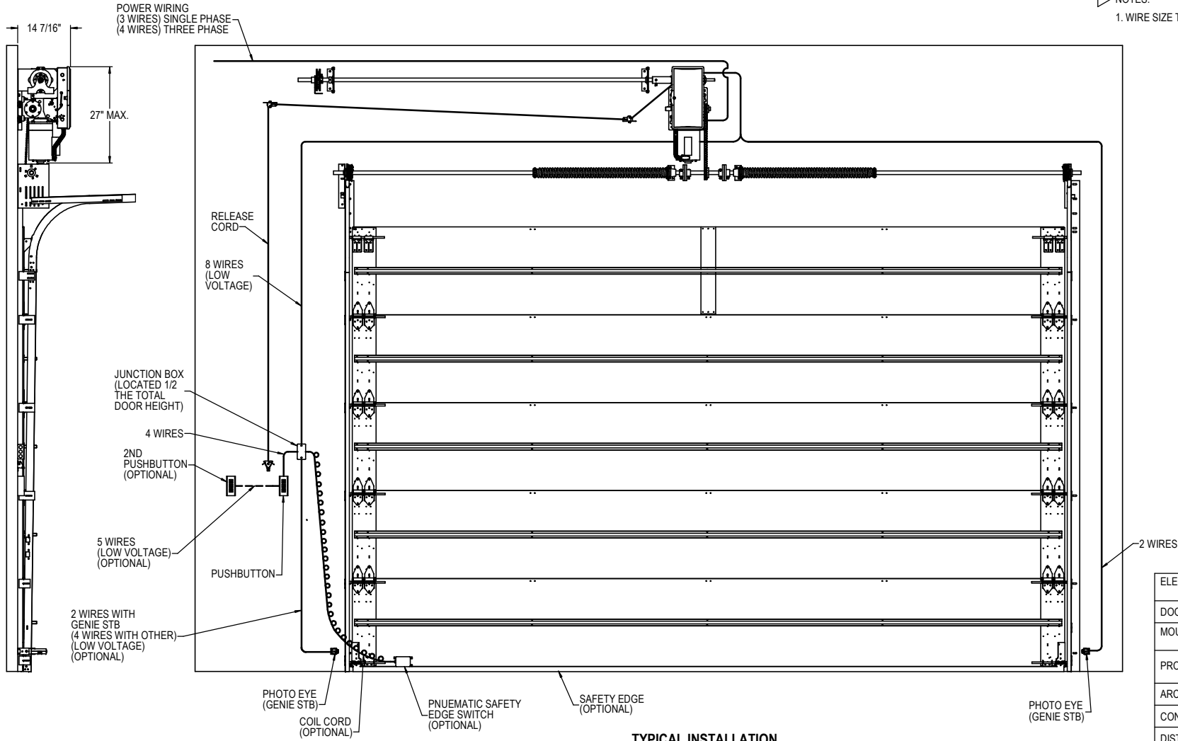
TYPICAL INSTALLATION
