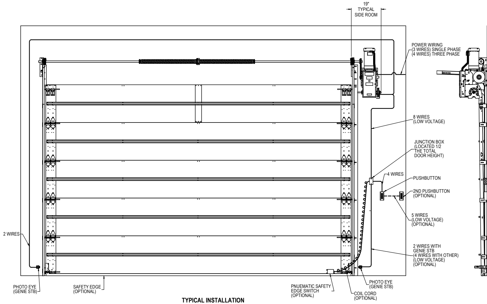
TYPICAL INSTALLATION
