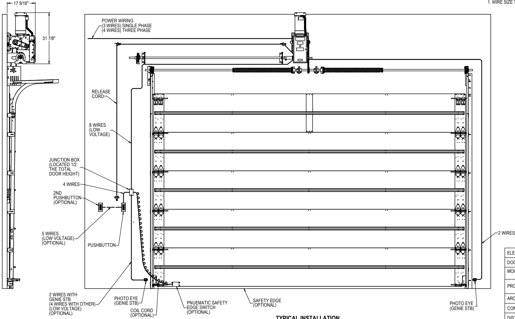
TYPICAL INSTALLATION
