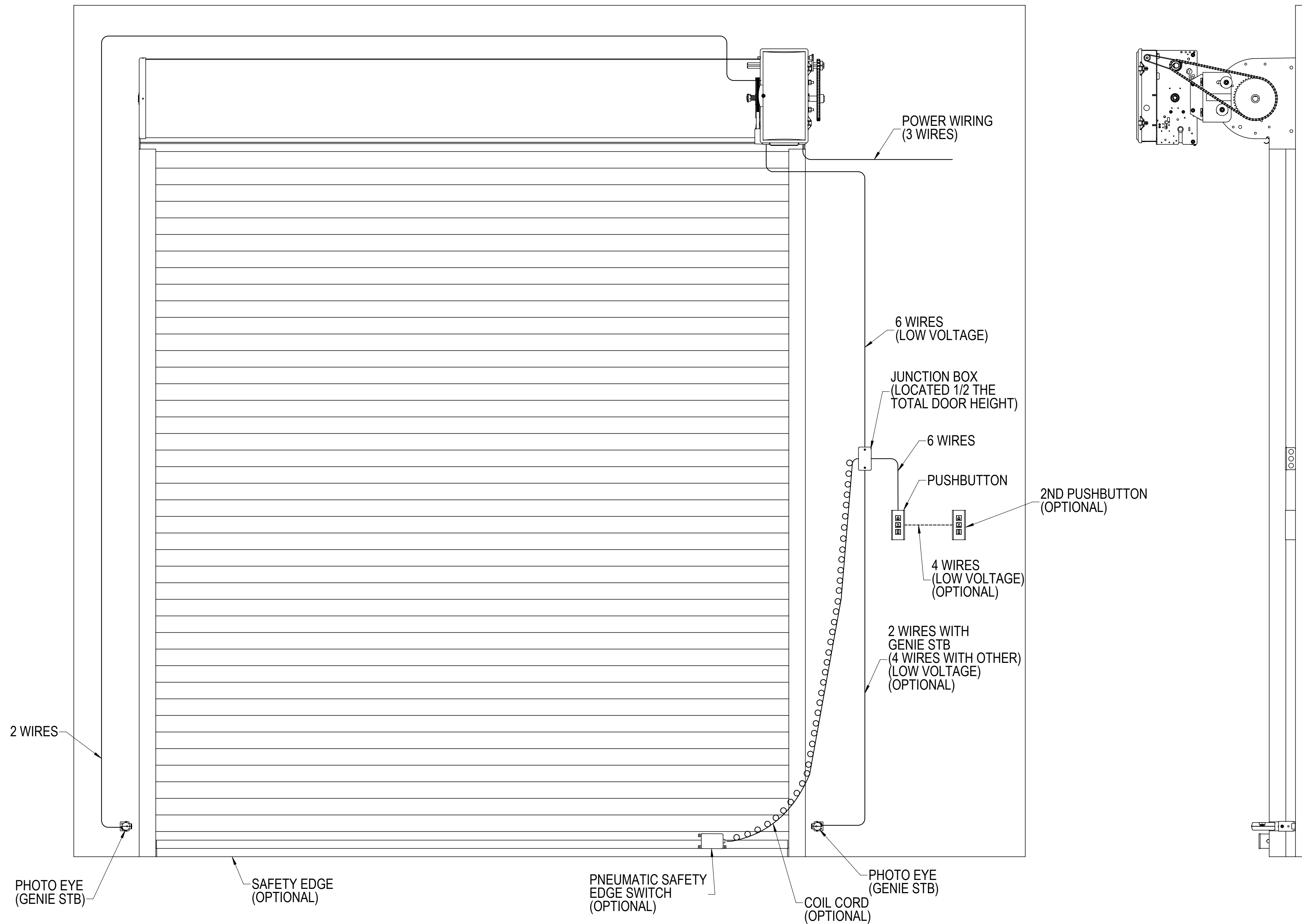
TYPICAL INSTALLATION
