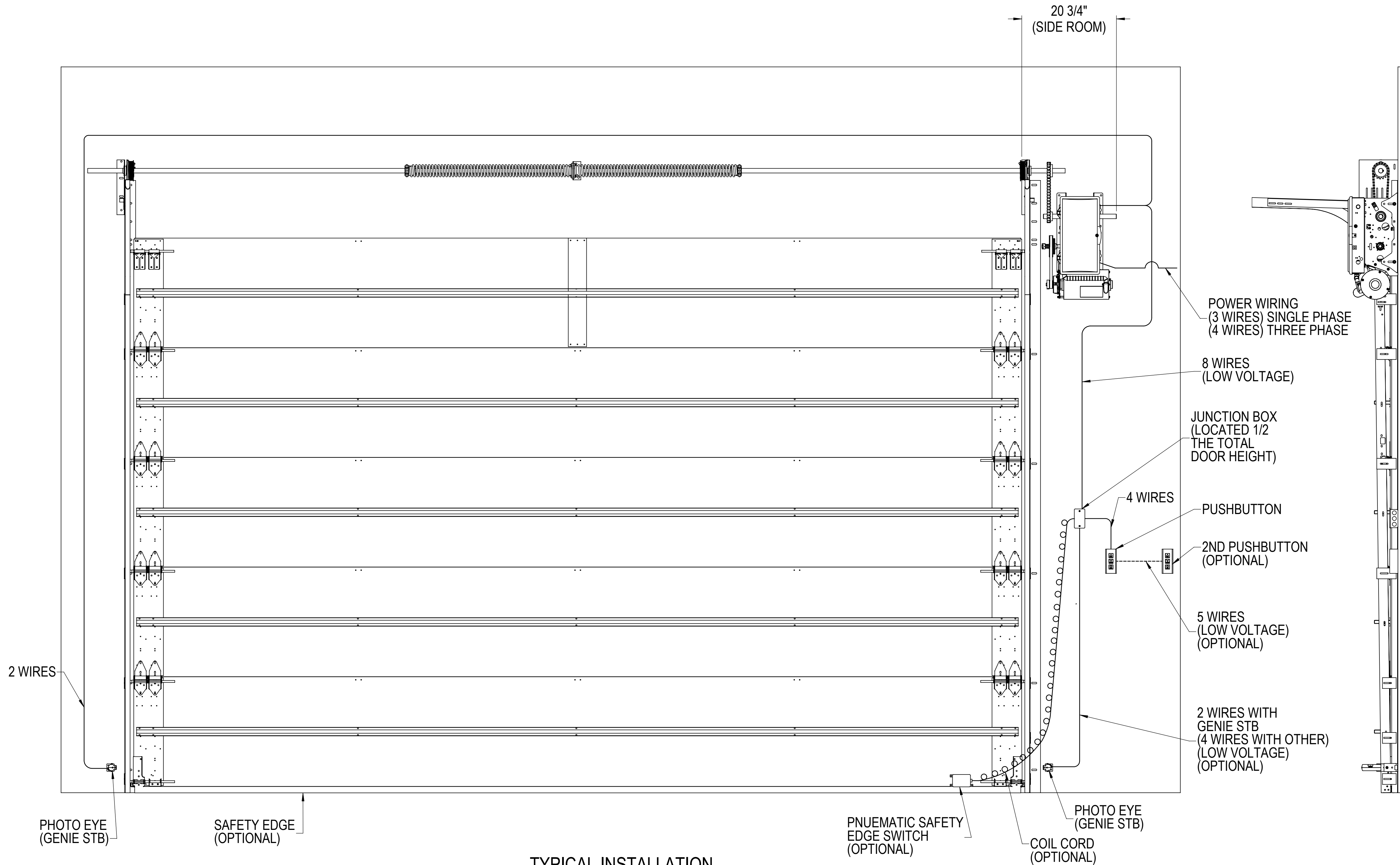
TYPICAL INSTALLATION
